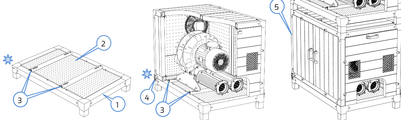
DIMENSION (SB-1)
