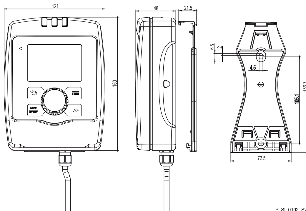
Fig. 1: Misure in mm
