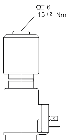
1 Fastening nut
