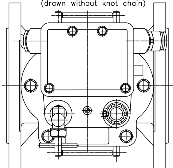
top view (drawn without knot chain)
