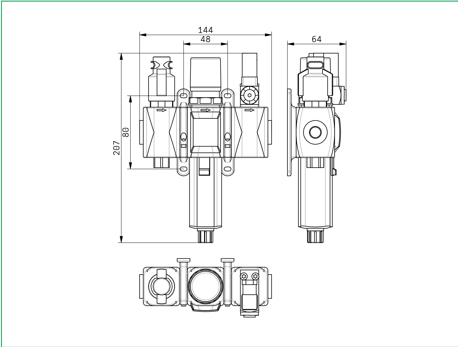
2D VIEW
