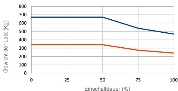
PM500FE 17m/min
