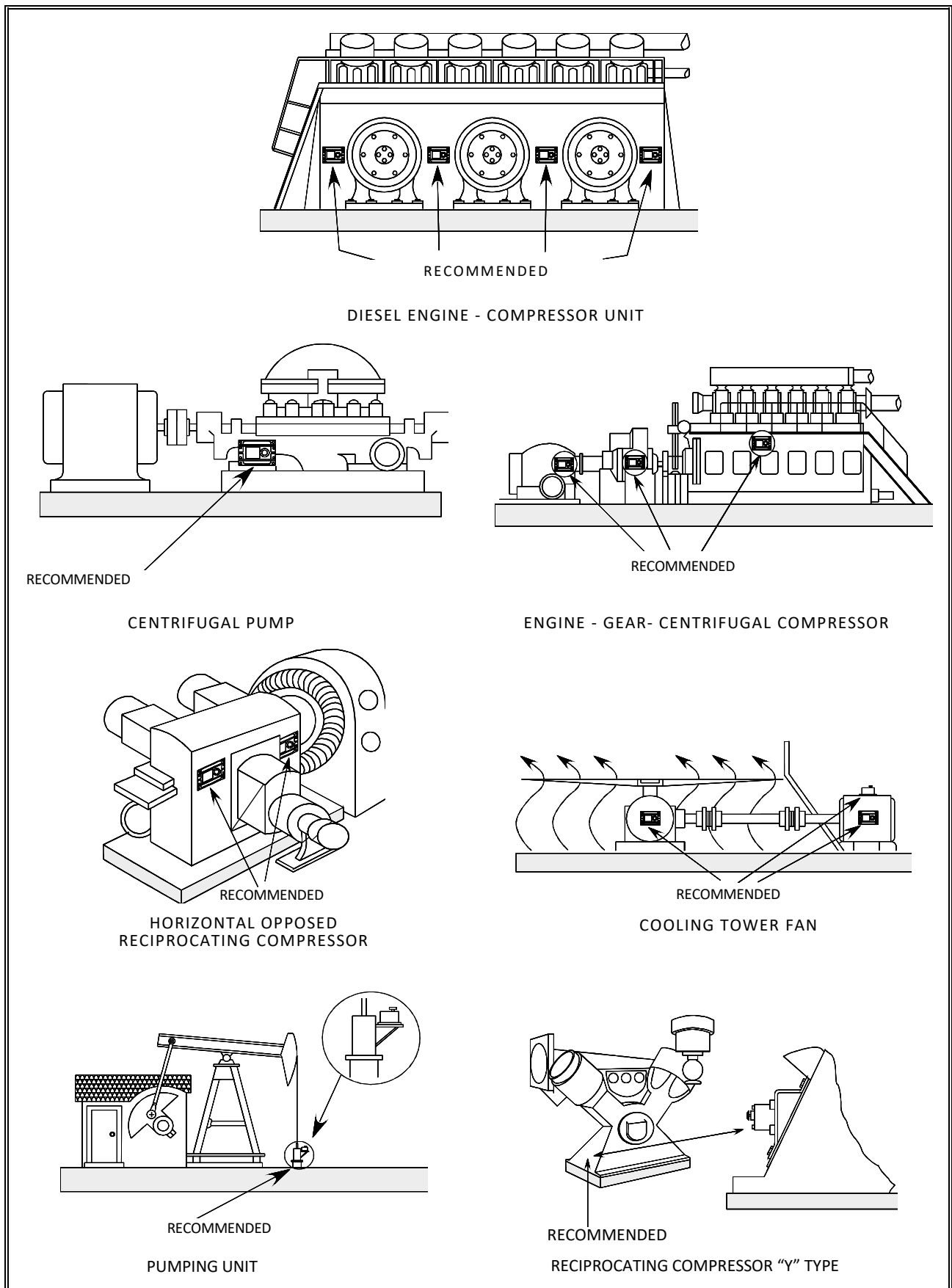
Figure 3-1. Methods of Mounting the Vibration switch, Model EURO366
