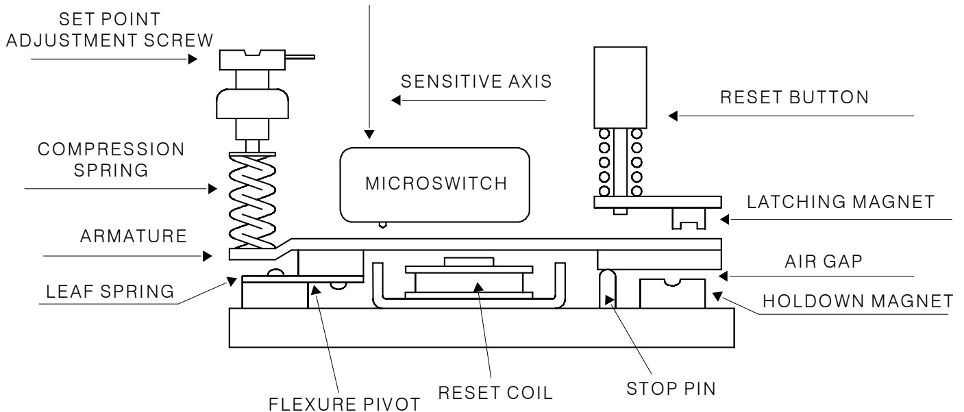
Figure 4-1. Operating Principle for the Vibration switch, Model EURO366.
