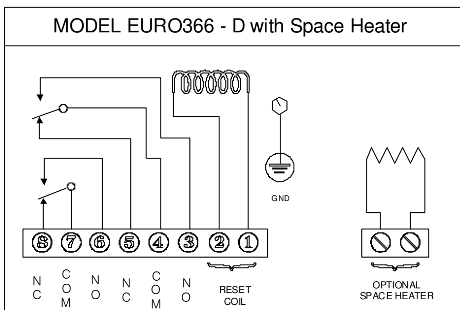
Figure 3-2. External Wiring for the Vibration switch, Model EURO 366.
