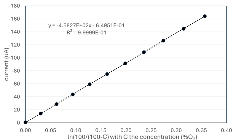
Figure 3 Linearity (0 - 30% Oxygen)
