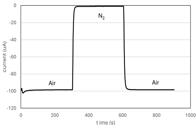
Figure 1 Response
