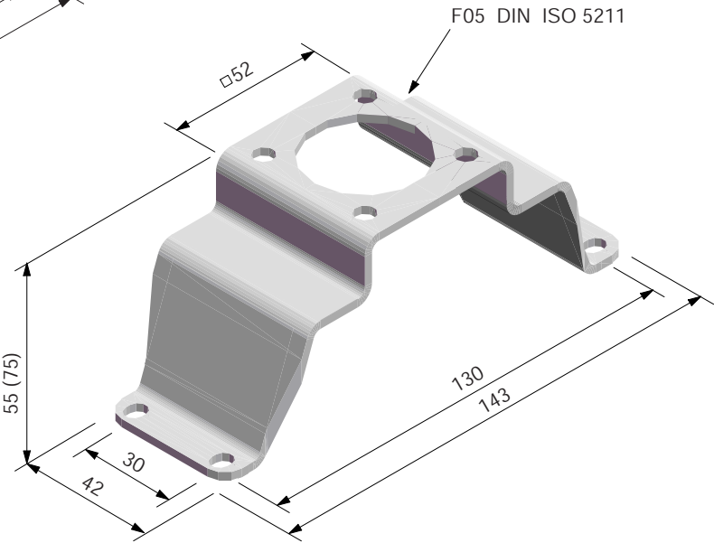
TCR-bracket TK1 (TK2) Bracket with hand lever interlock suitable for actuators size 1 (size 2) according to VDI/VDE 3845
