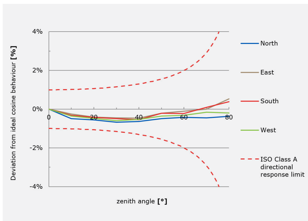
Figure 2.1.2 Example of a directional response of a SR200 pyranometer at 4 azimuth angles, compared to spectrally flat Class A (secondary standard) limits for the maximum directional error.
