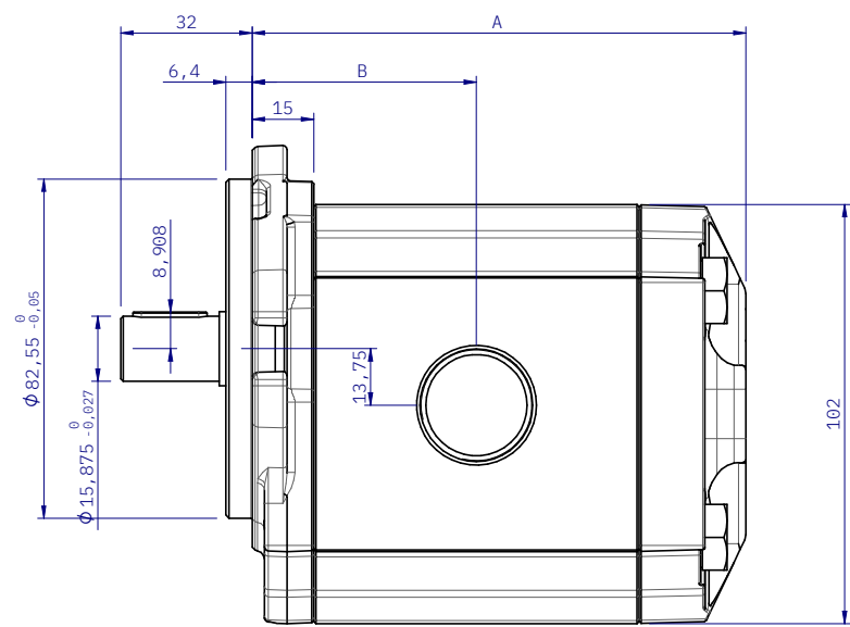
SAE J1926-1 (ISO 11926-1) Straight thread O-ring Port -12
