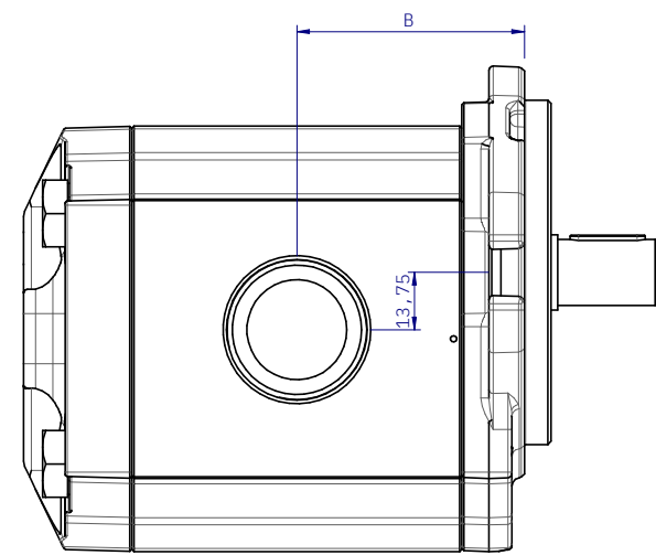
SAE J1926-1 (ISO 11926-1) Straight thread O-ring Port -16
