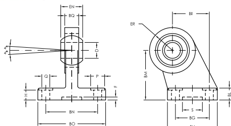
BRIDE AVANT/ARRIÈRE (MF1-MF2)
