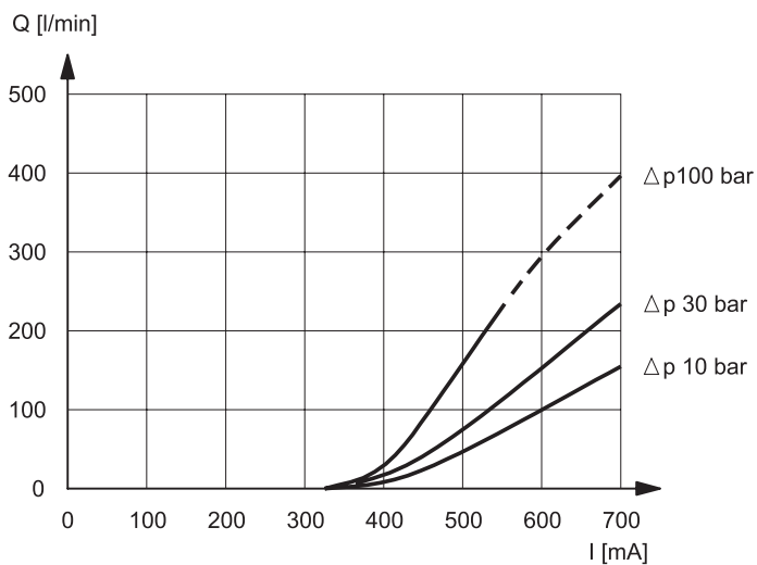
SPOOL TYPE 93
