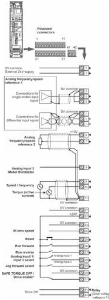
M700/M701: Default Control Connections
