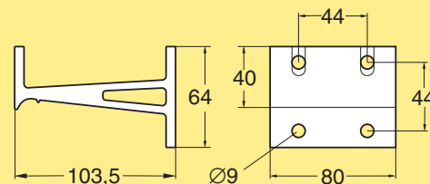
Beam support bracket, Type CU
