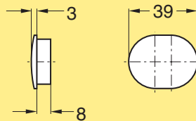
Nut cover plug for elongated hole
