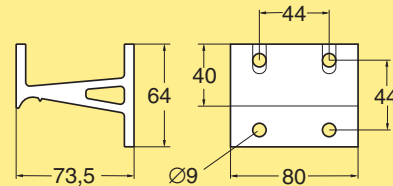
Beam support bracket, Type CU
