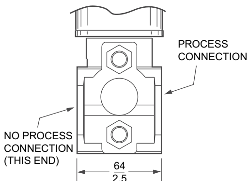
OPTIONAL IEC 61518 CONSTRUCTION SINGLE ENDED PROCESS COVER OPTIONS -D5, -D7, -D9
