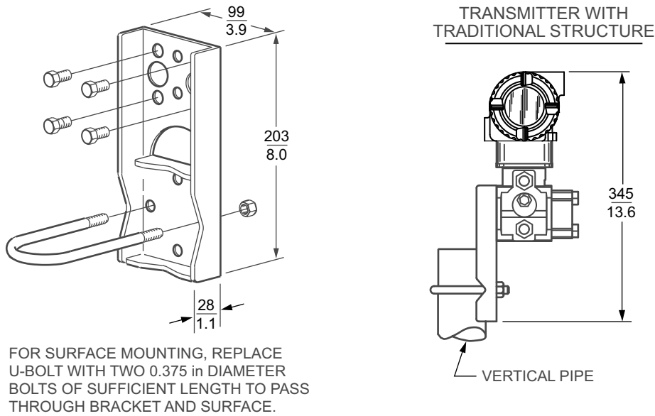
Figure 30 - DP Transmitters with Option -M3 (Universal Style Mounting Bracket Kit)
