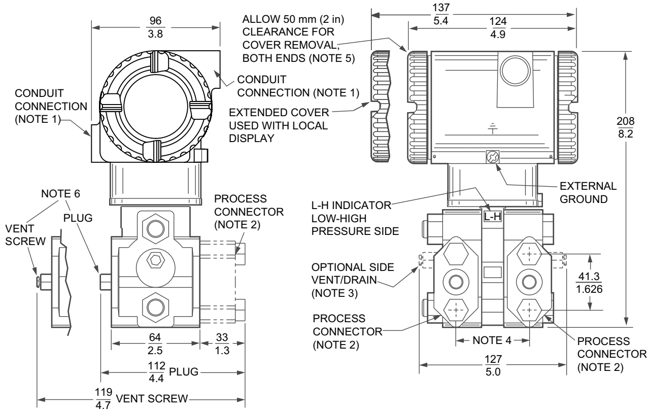
Figure 27 - DP Transmitters with Traditional Structure
