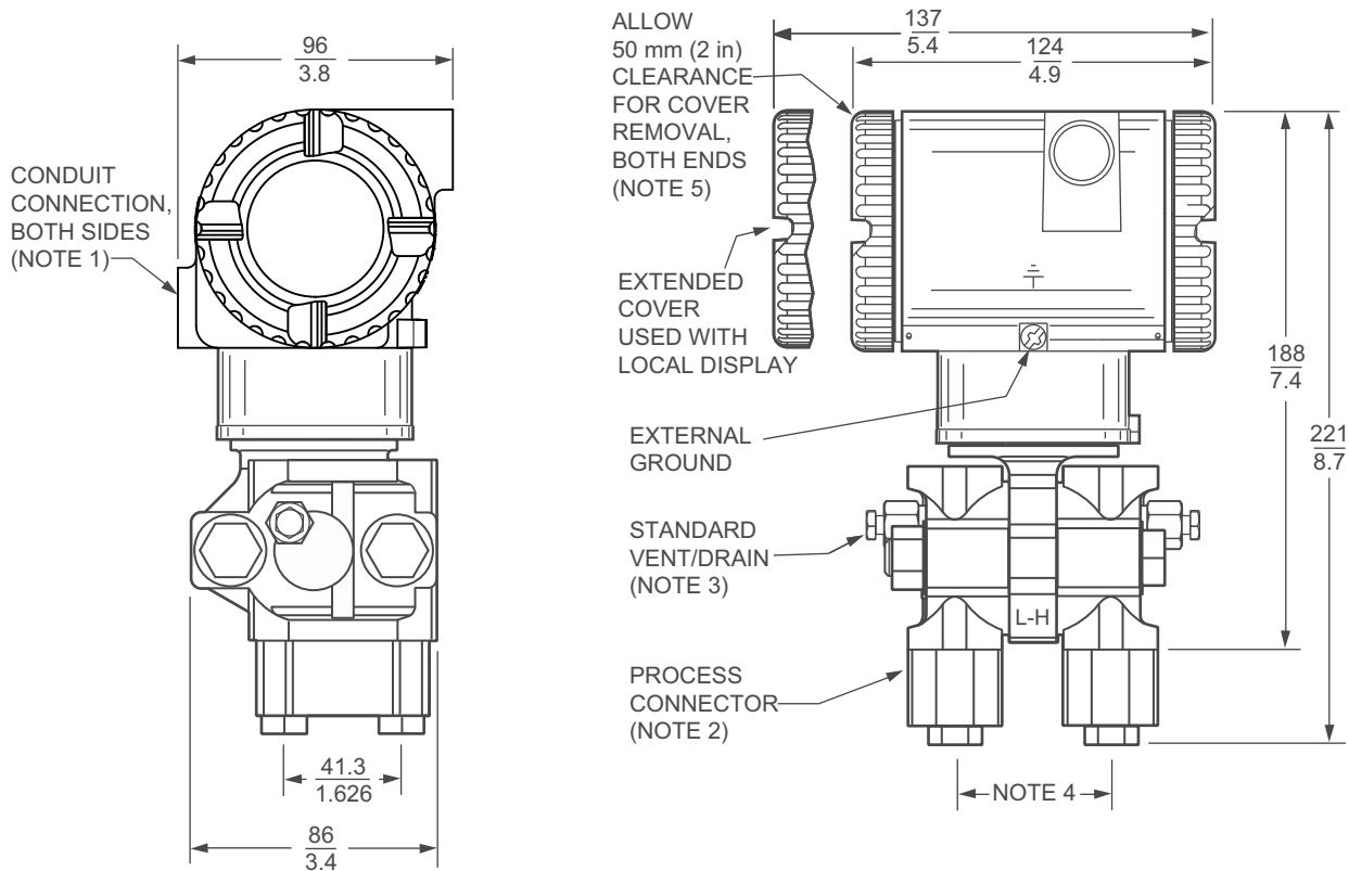
Figure 28 - DP Transmitters with Low Profile 1 (LP1) Structure
