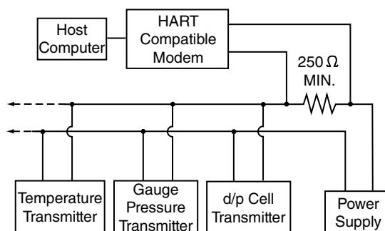
Figure 18 - Typical Multidrop Functional Block Diagram
