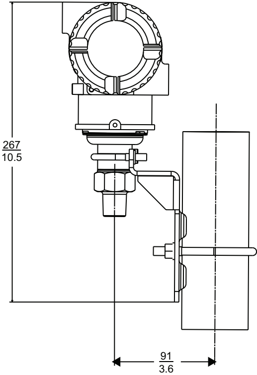
Figure 22 - Flameproof Direct Connect AP/GP Transmitters with Options -M7 and -M8
