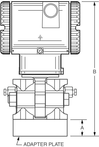
Figure 31 - DP Transmitters with LP1 Structure Mounted on a Coplanar™ Manifold
