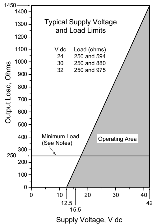
Figure 15 - 4 to 20 mA Output Supply Voltage vs Output Load
