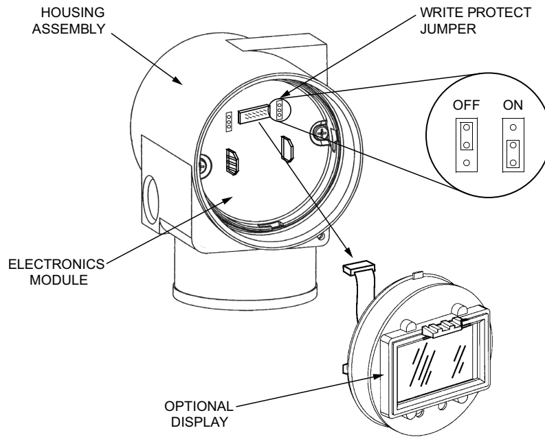
Figure 16 - Write Protect Jumper
