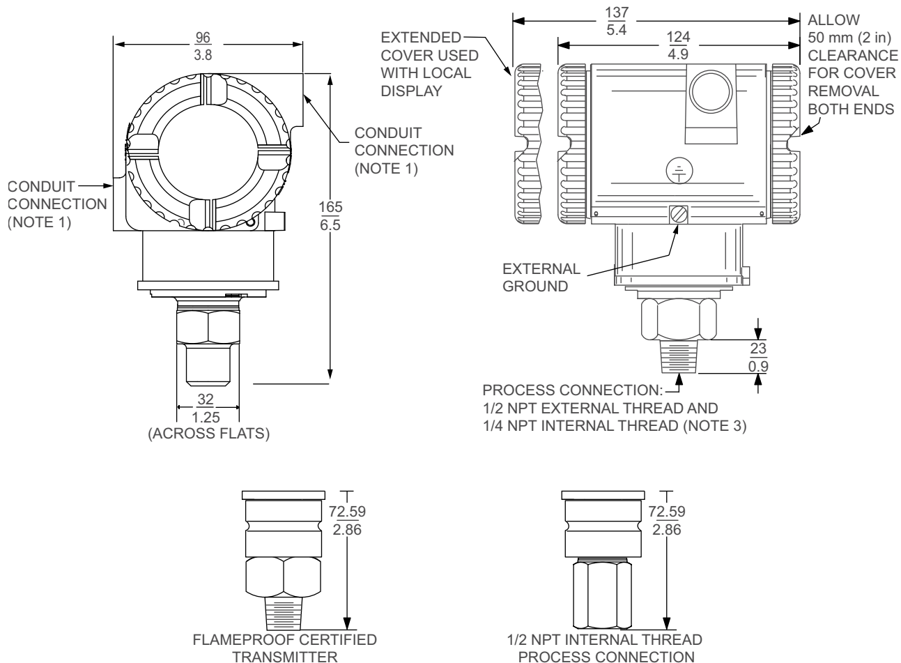
Figure 19 - Direct Connect AP/GP Transmitters
