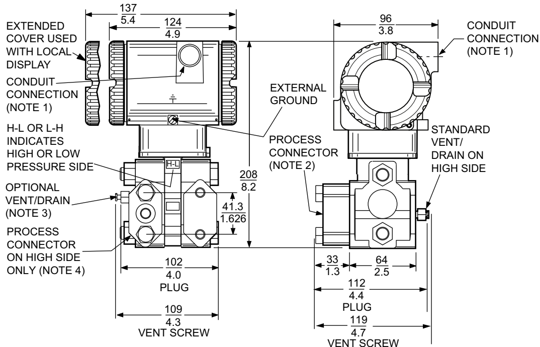
Figure 23 - Biplanar AP/GP Transmitters
