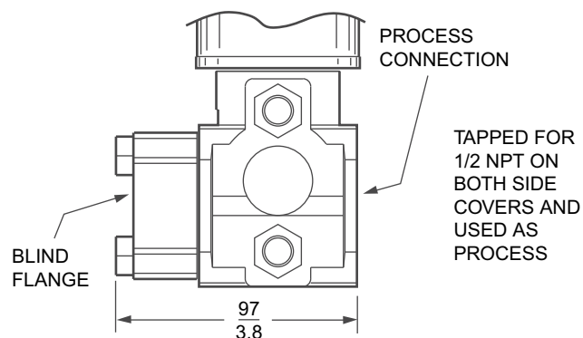
OPTIONAL IEC 61518 CONSTRUCTION DOUBLE ENDED PROCESS COVER OPTIONS -D6, -D8
