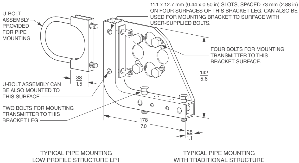
Figure 30 - DP Transmitters with Option -M3 (Universal Style Mounting Bracket Kit)
