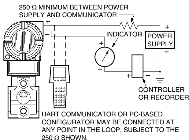
Figure 17 - 4 to 20 mA Output Functional Block Diagram, Point-to-Point Communications
