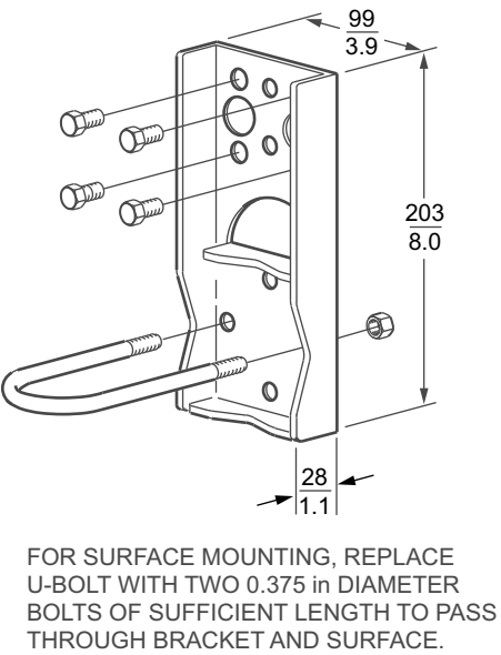
Figure 25 - Biplanar AP/GP Transmitters with Options -M0 and -M9 (Standard Stainless Steel or Painted Steel Bracket)
