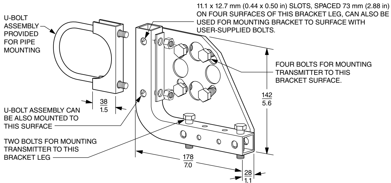
Figure 26 - Biplanar AP/GP Transmitters with Option -M3 (Universal Bracket)
