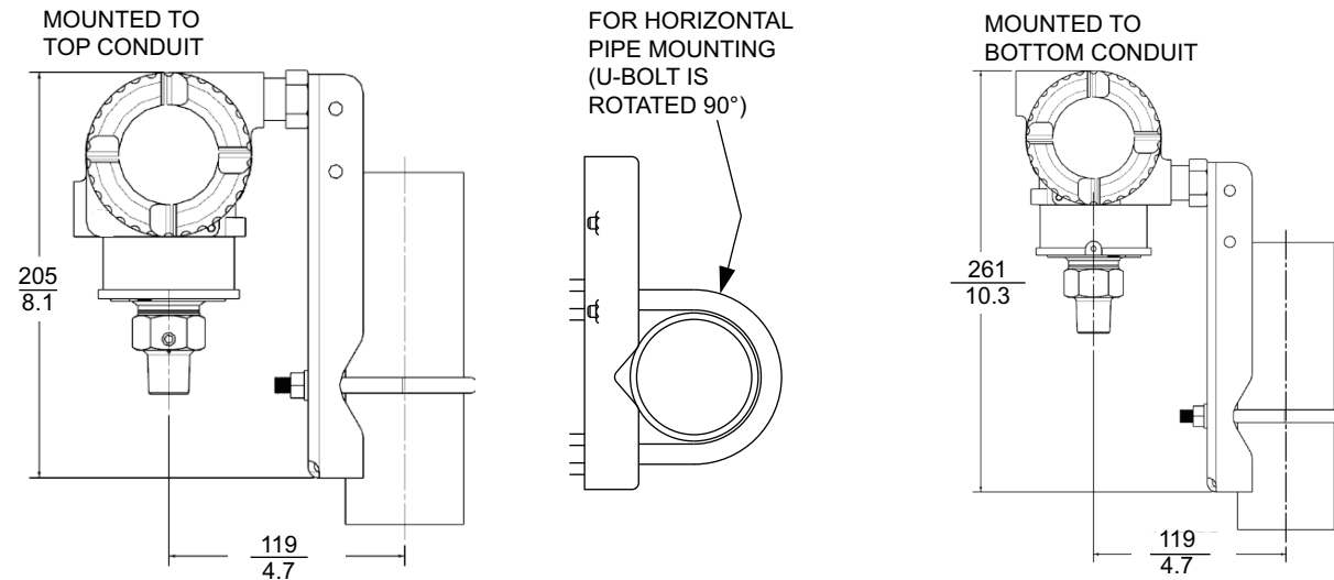
Figure 21 - Direct Connect AP/GP Transmitters with Options -M1, -M2, -M5, and -M6
