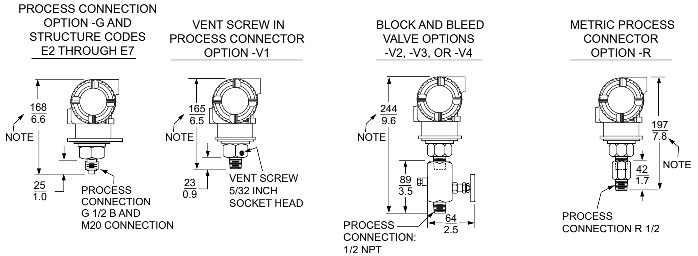
Figure 20 - Direct Connect AP/GP Transmitters with Options -G, -V1, -V2, -V3, -V4, and -R
