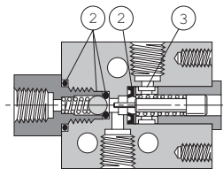
3-Way Poppet
