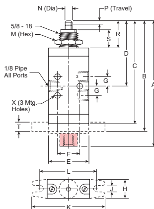
One-Way Tripper Operated
