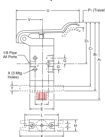
Hand Lever Operated
