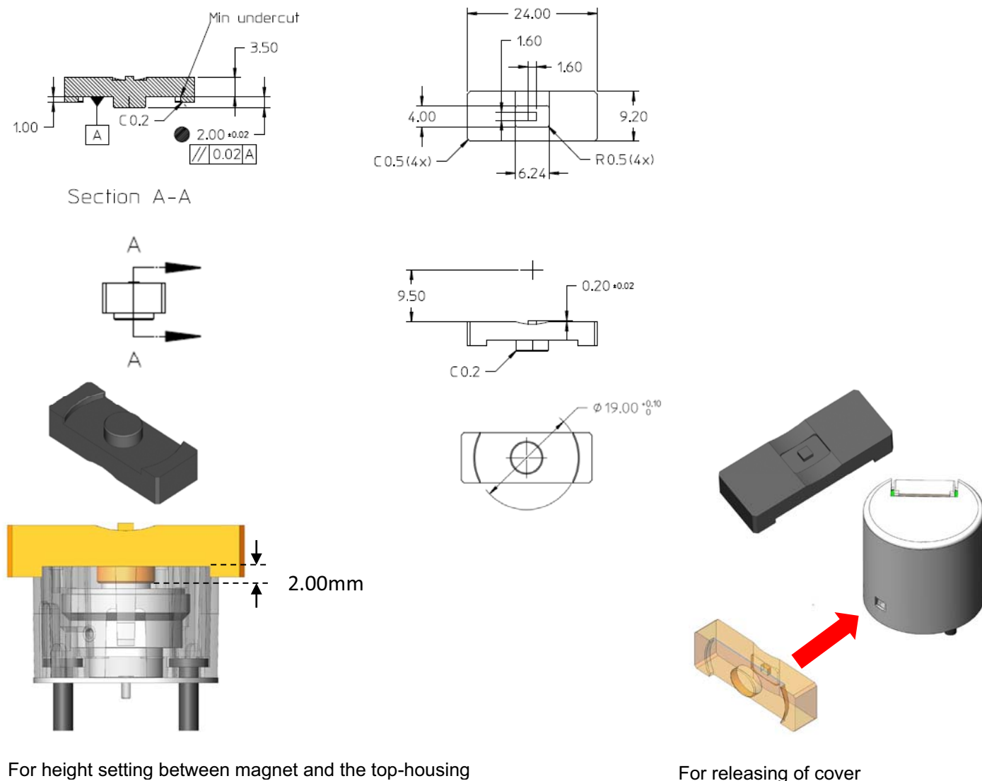
Figure 3: Set Height and Housing Latch Release Tool
