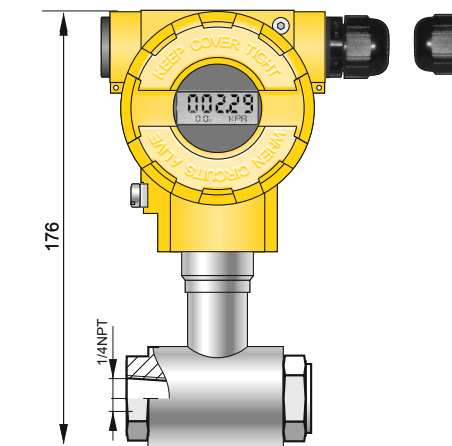
Transmitter APR-2000ALW Version with PN type process connection.
