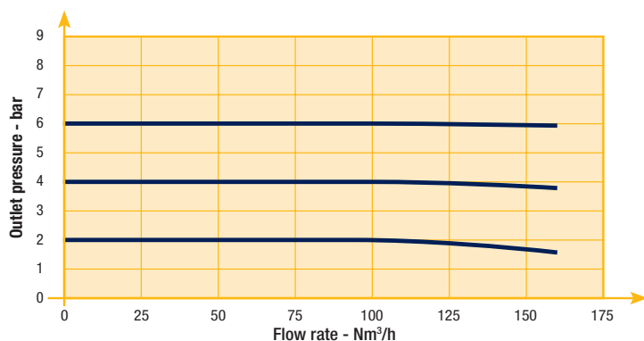
Flow Curve 1"
