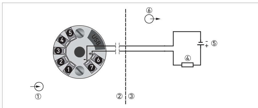
Figure 4-2: Connection diagram
