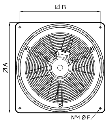
QCM-ATEX 200-560
