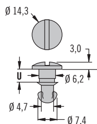
Oval, fenda
