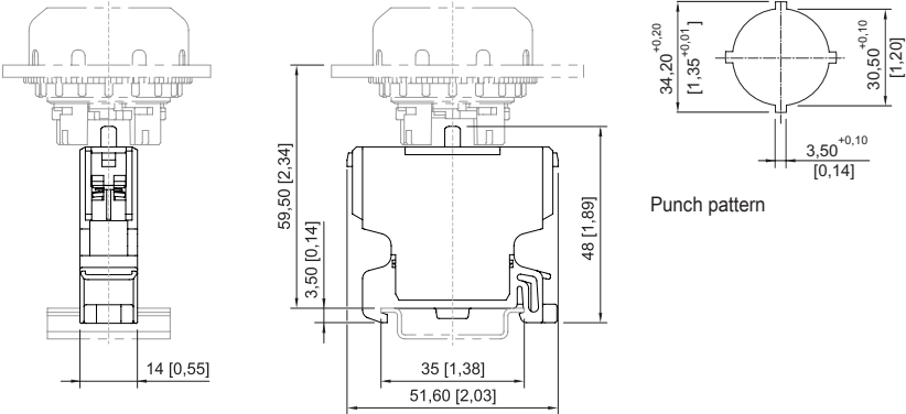
Contact element for installation on mounting rail
