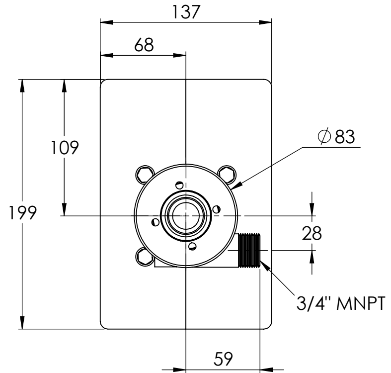
BOTTOM VIEW
