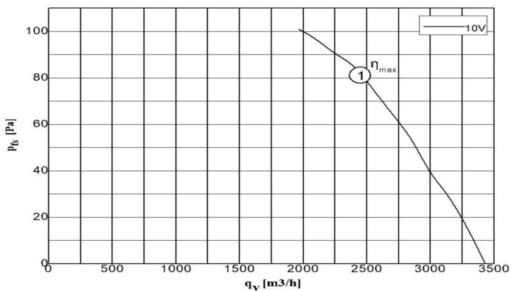
Curva caratteristica / Characteristic curve
