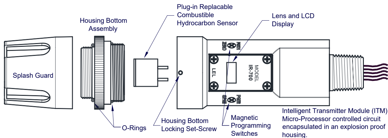
Figure 18 Sensor Assembly
