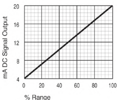
Figure 3 Response Curve
