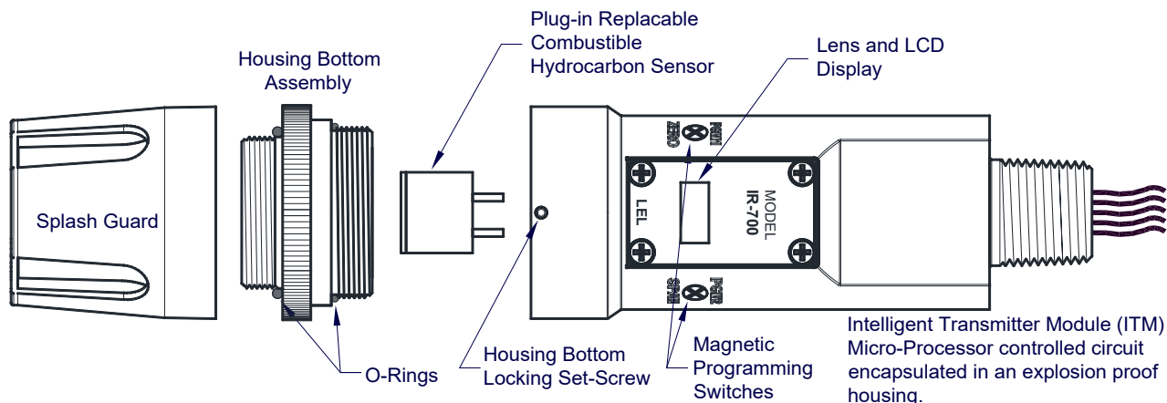
Figure 6 Sensor Assembly Breakaway
