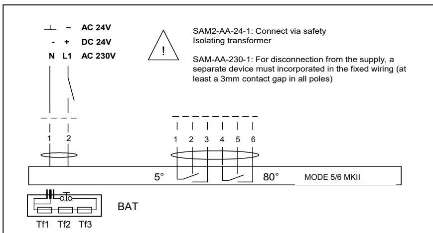
Wiring Diagram
