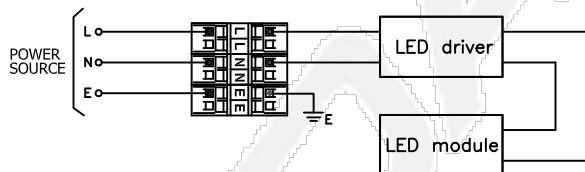
CIRCUIT DIAGRAM
