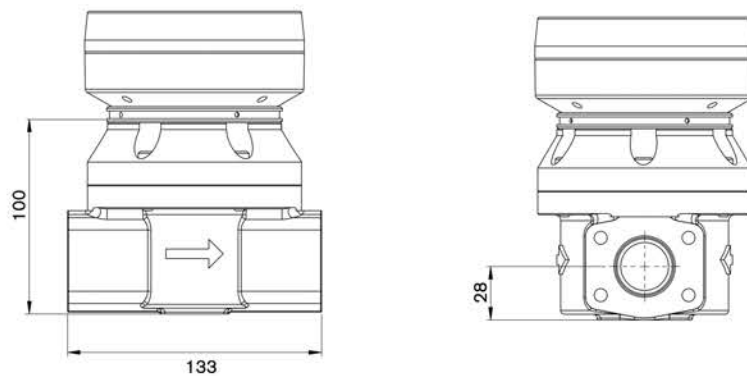
TYPE 4 MECHANICAL REGISTER - HEAVY DUTY
