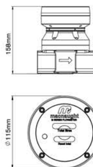
TYPE 3 MECHANICAL REGISTER - STANDARD
