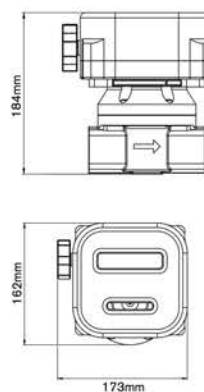
TYPE 4 MECHANICAL REGISTER - HEAVY DUTY
