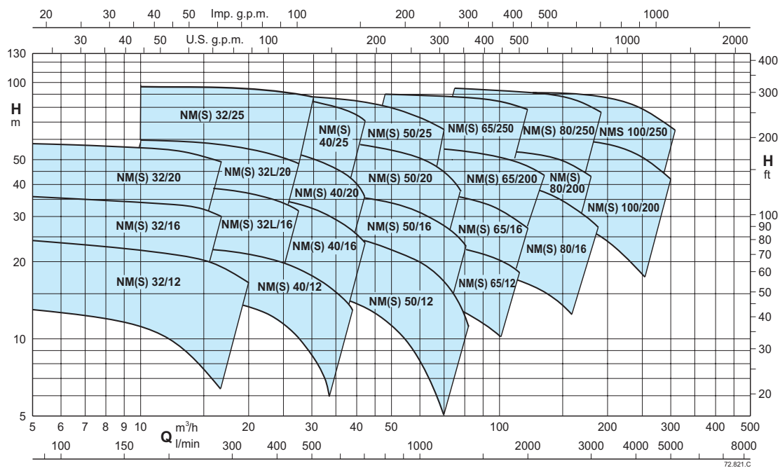
Performance n ≈ 3450 1/min
