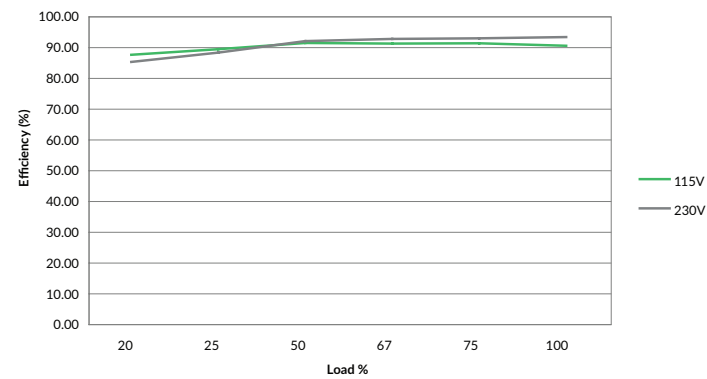
Figure 4 GCS250PS24
