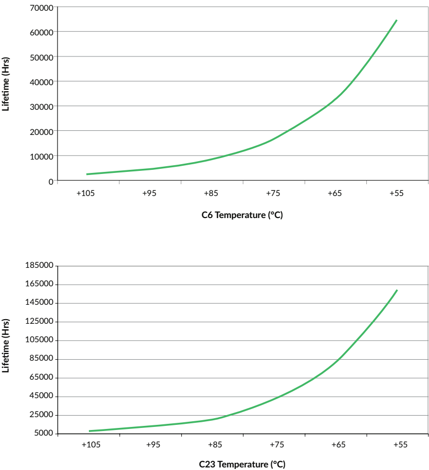
Estimated service life vs component temperature
