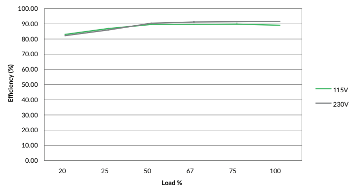
Figure 5 GCS250PS48
