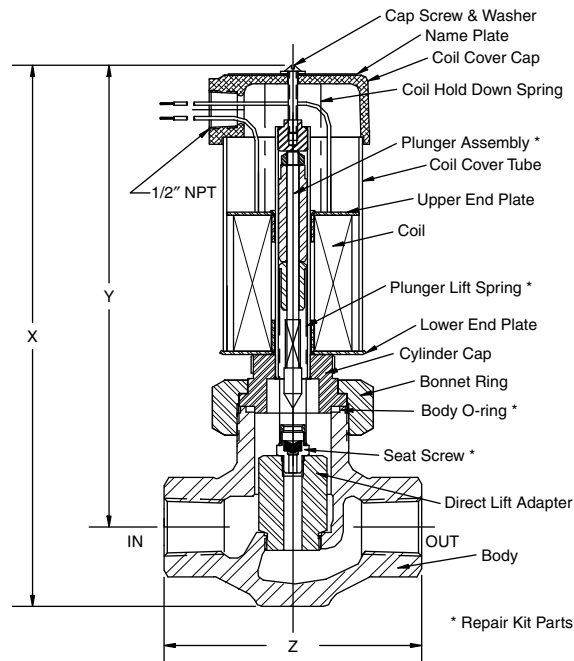
Normally open 16201 1/2" valve, shown with a NEMA 1 coil housing and a soft seat
