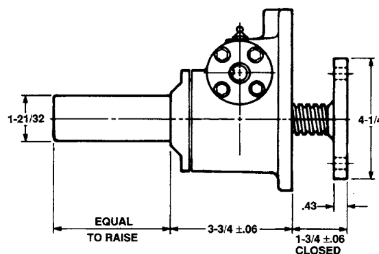
Inverted: M-9001
