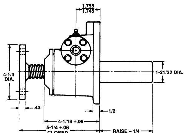
Upright: M-9002
