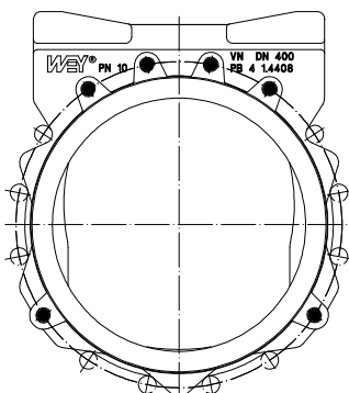
DN 400
