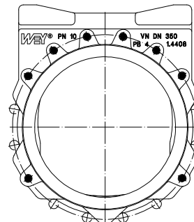
DN 350
