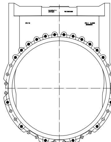
DN 1400
