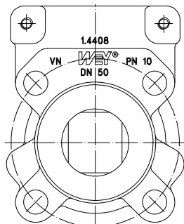
DN 50
