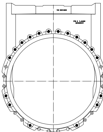
DN 1200
