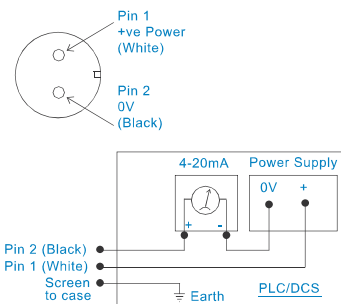
Connection Details
