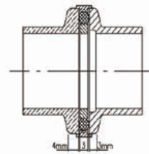
Glass to metal connection
