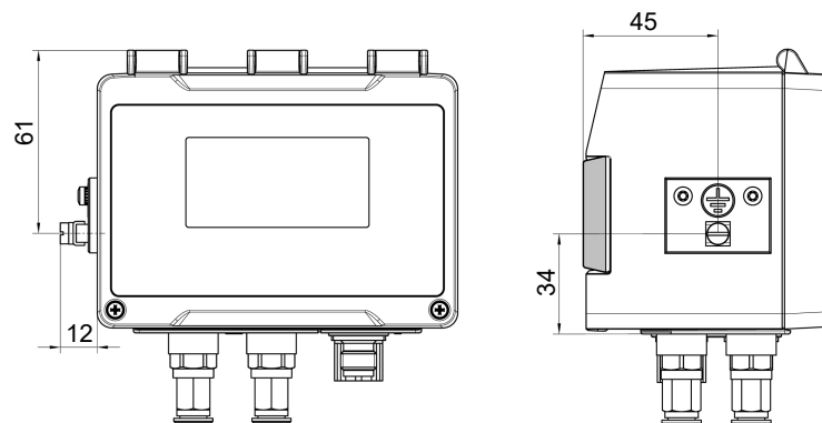
Fig. 6: Dimension drawing ATEX
