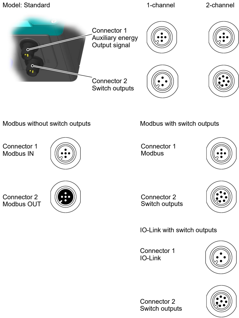
Fig. 3: Electric connections
