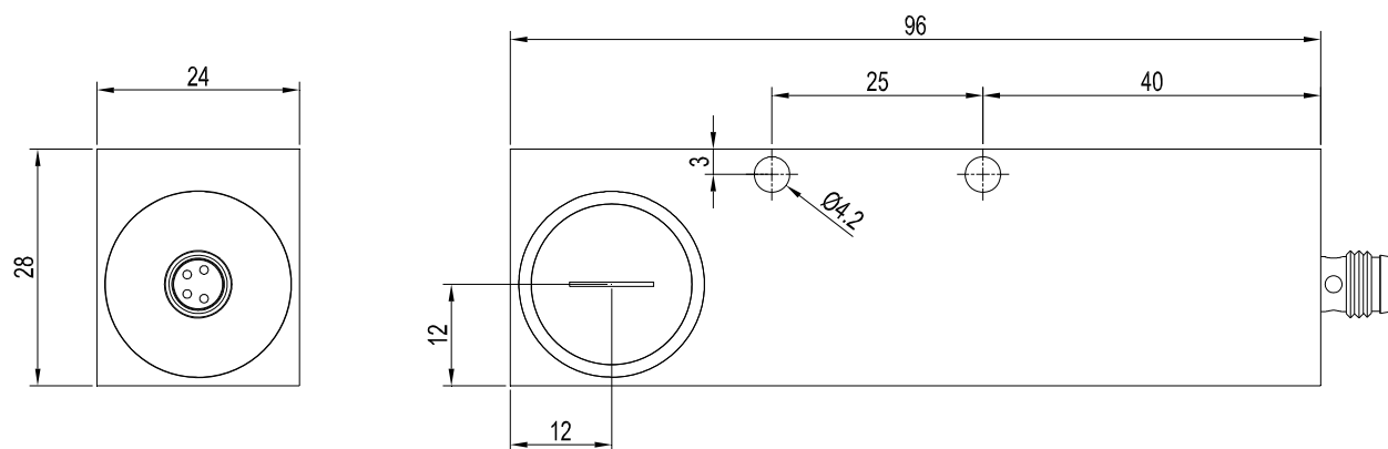
A-LAS-24/90-...-R (Receiver):
