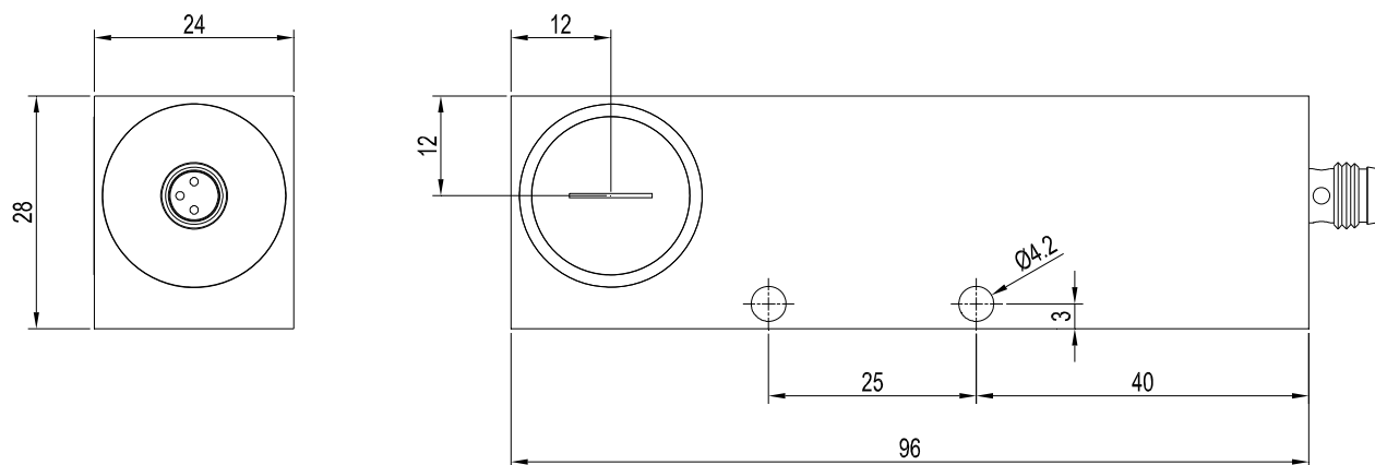
A-LAS-24/90-...-T (Transmitter):
