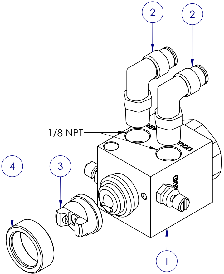
EXPLODED VIEW
