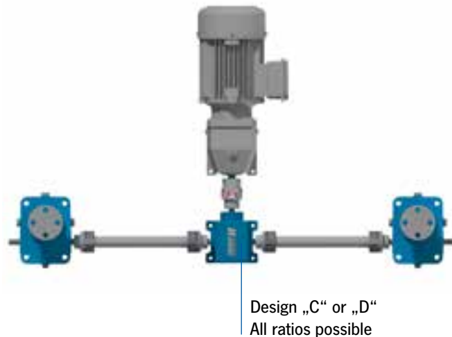
Schematic view 2.3
