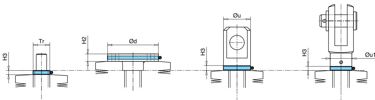
Protection boot fasteners – gear box area
