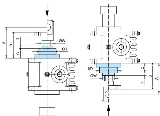
HSE type 1, compression load
