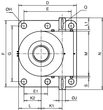
Size 150.1 and 200.1
