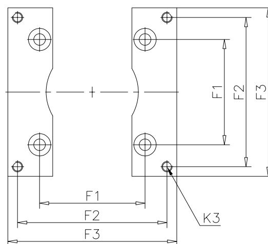
Mounting brackets (A1)
