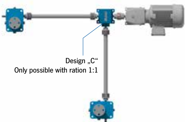
Schematic view 2.4
