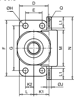
Size 75
