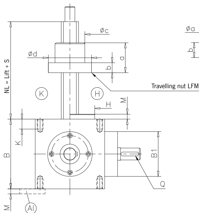
Head I
