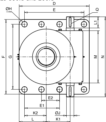
Size 150.1 and 200.1
