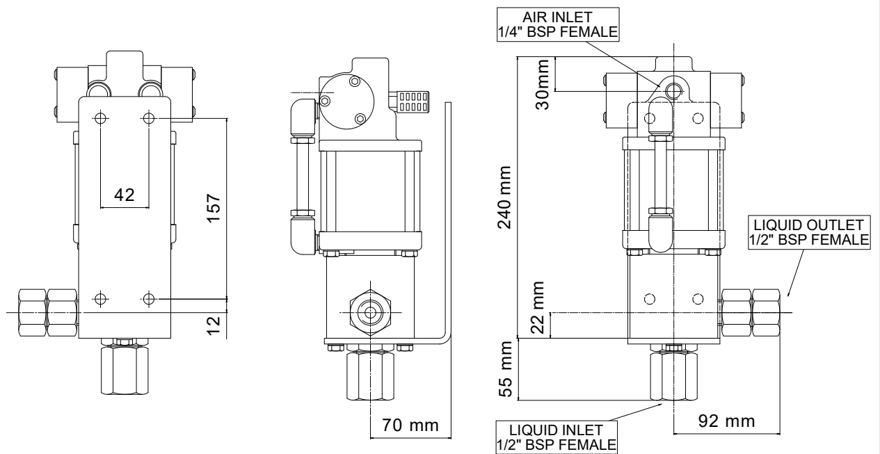
The Trojan Type 'J' Ratio 11:1, Version 'FS'
