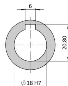
HOLLOW OUTPUT SHAFT
