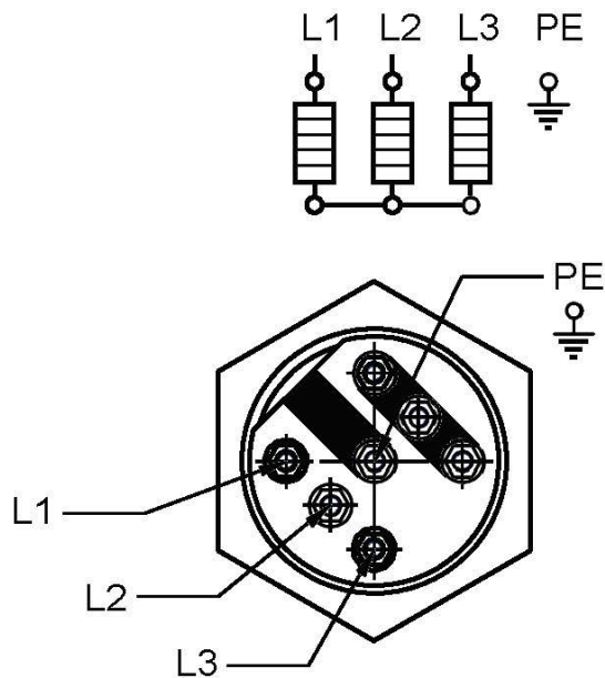
Circuit diagram 3 phases AC
