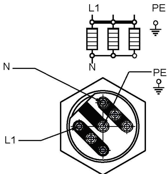
Circuit diagram 1 phase AC
