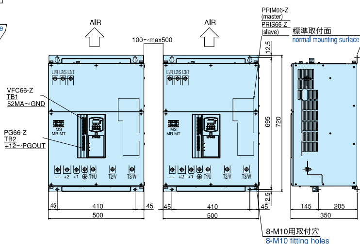
Non-standard type ( Cooling fin is used installing outside)
