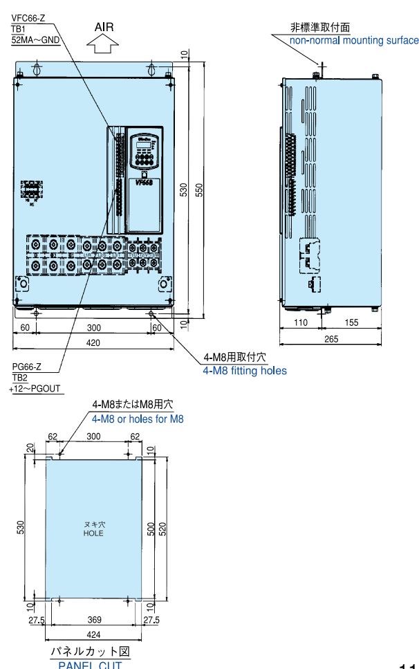
Non-standard type (Cooling fin is used installing outside)
