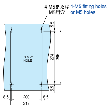
非標準取付穴加工図 Non-standard mounting hole manipulation figure
