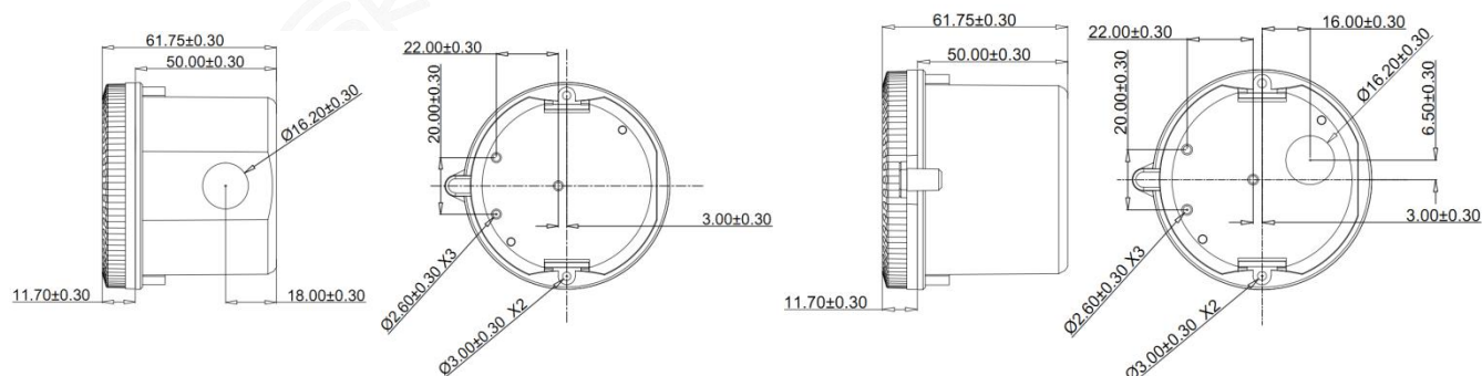
Opening holes on the side
