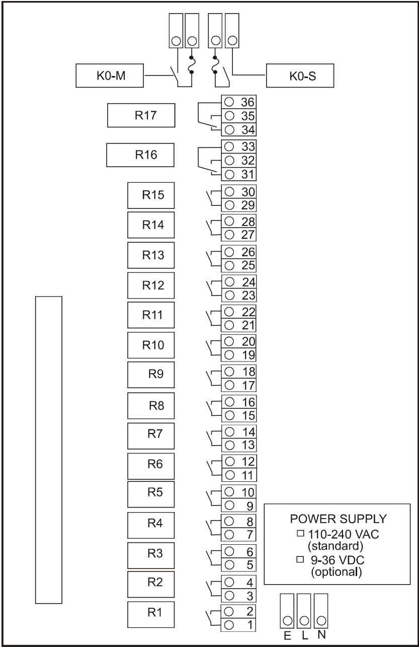
Figure 18: CT24-17 Relays and Terminals
