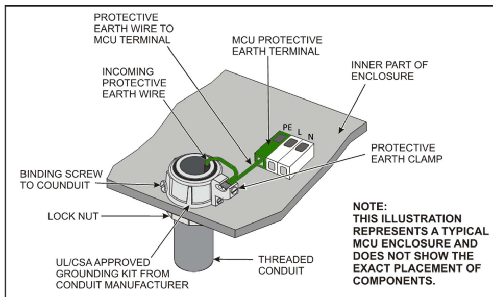
Figure 20: Metallic Conduit Installation
