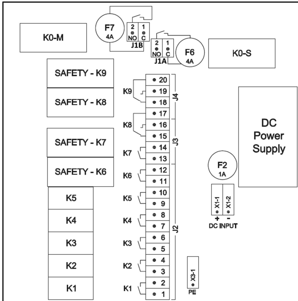
Figure 17: CT24-9-ASO DC Version Relays and Terminals
