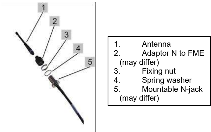
Figure 23: Remote Antenna Parts
