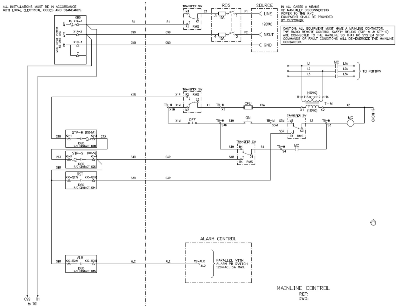
Figure 21 Example Typical non-PLd Mainline and Manual Remote Transfer Drawing
