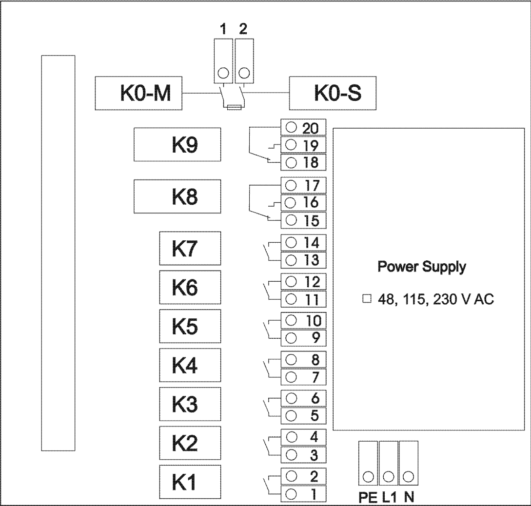
Figure 15: CT24-9 Relays and Terminals
