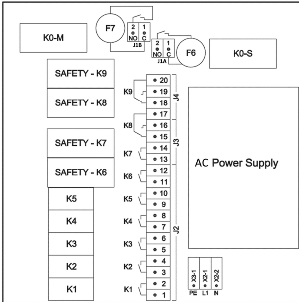
Figure 16: CT24-9-ASO AC Version Relays and Terminals
