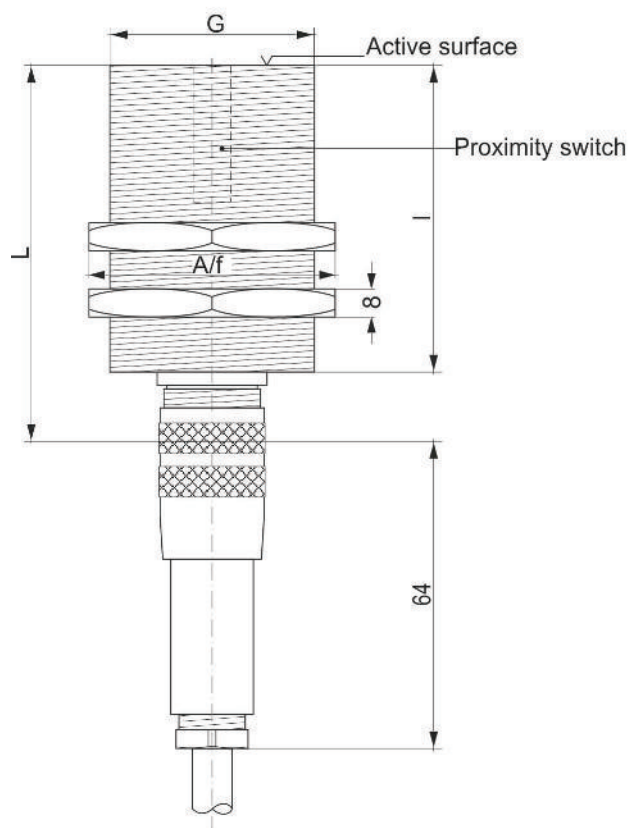
BDIF Sheet Metal Thickness Sensor cylindrical, threaded
