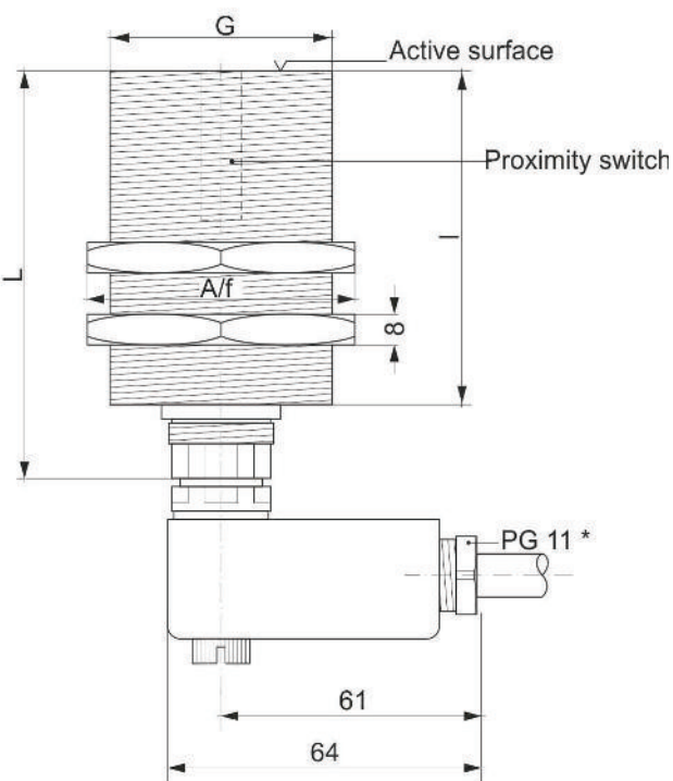
BDIF Sheet Metal Thickness Sensor cylindrical, threaded
