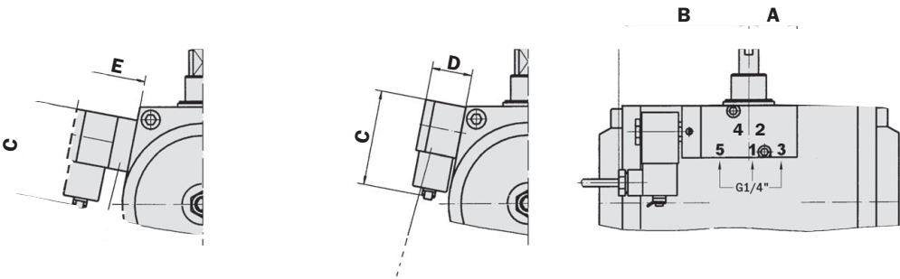
with NAMUR-valve adapter (VPN) for actuator sizes 046 to 096
