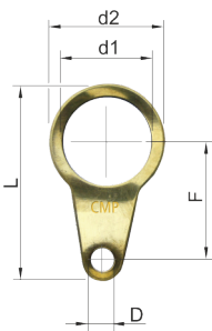
Dimensional Drawings (All Dimensions in mm [inches]) – Subject to Alterations
